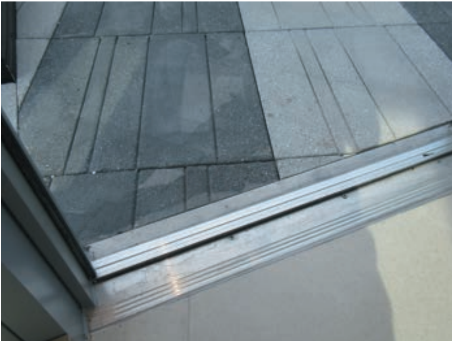
Figure 4. Thermally broken door threshold with saddle profile containing vertical element with gaskets that integrate with jamb gasketing.
